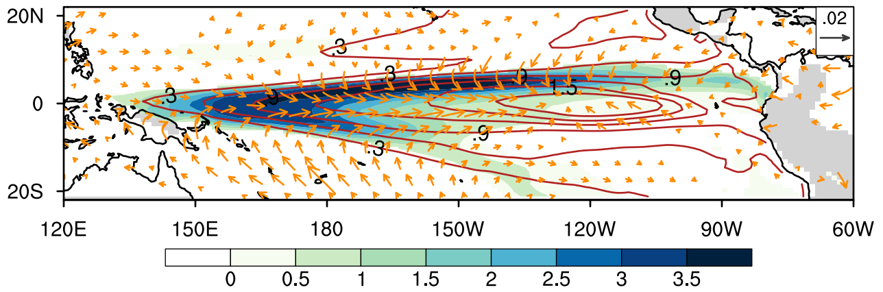
NorESM2-MM historical Nino 3.4 reg ts , wind-stress & pr
