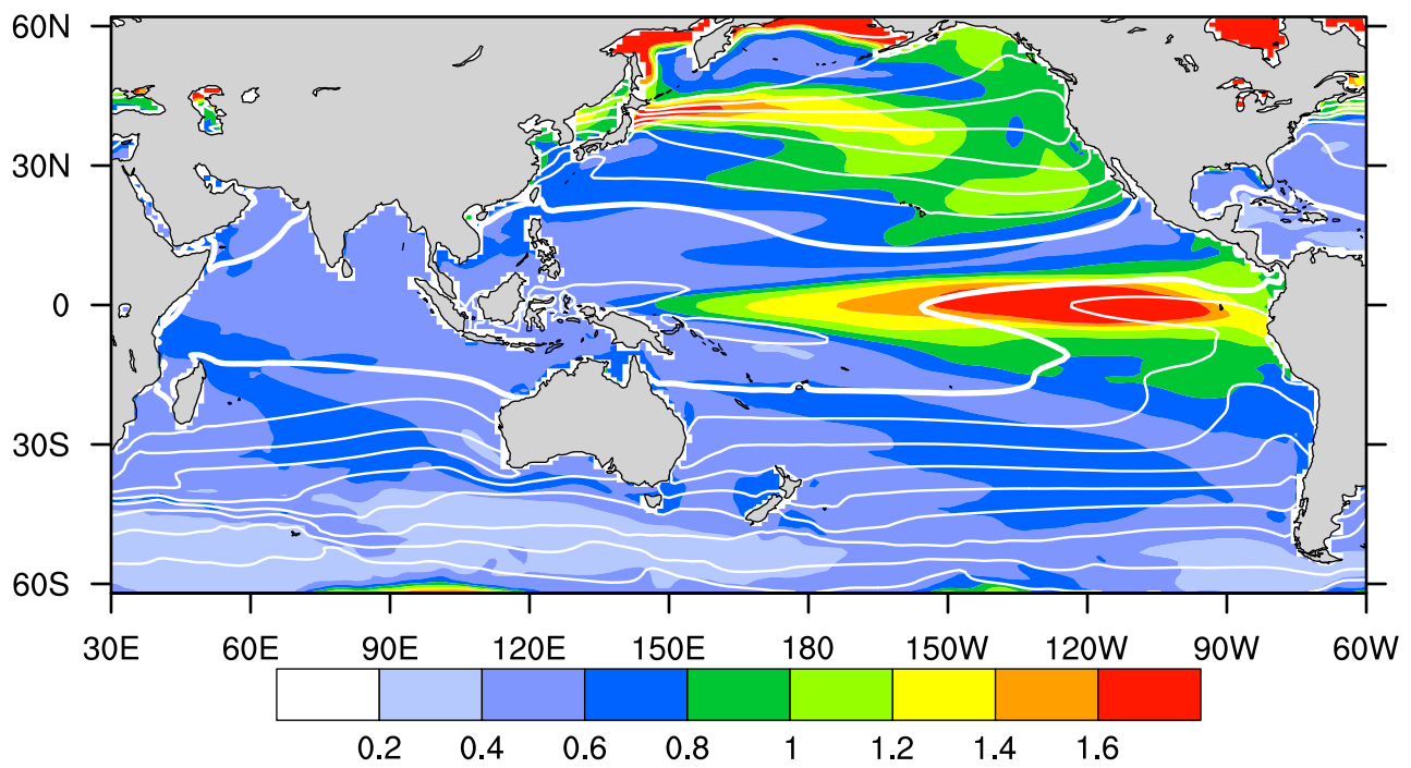
NorESM2-MM historical monthly STD. (1900-2014)
