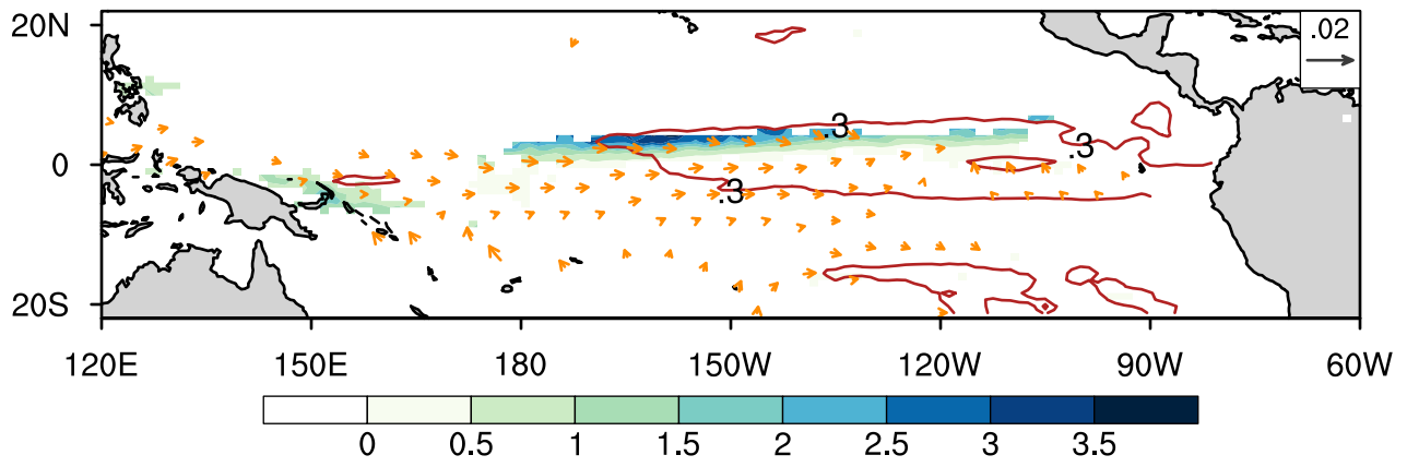
NorESM13-hires 1950-control Nino 3.4 reg ts , wind-stress & pr
