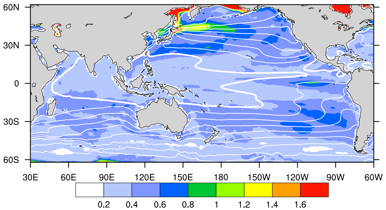
NorESM13-hires 1950-control monthly STD. (61-73) degC
