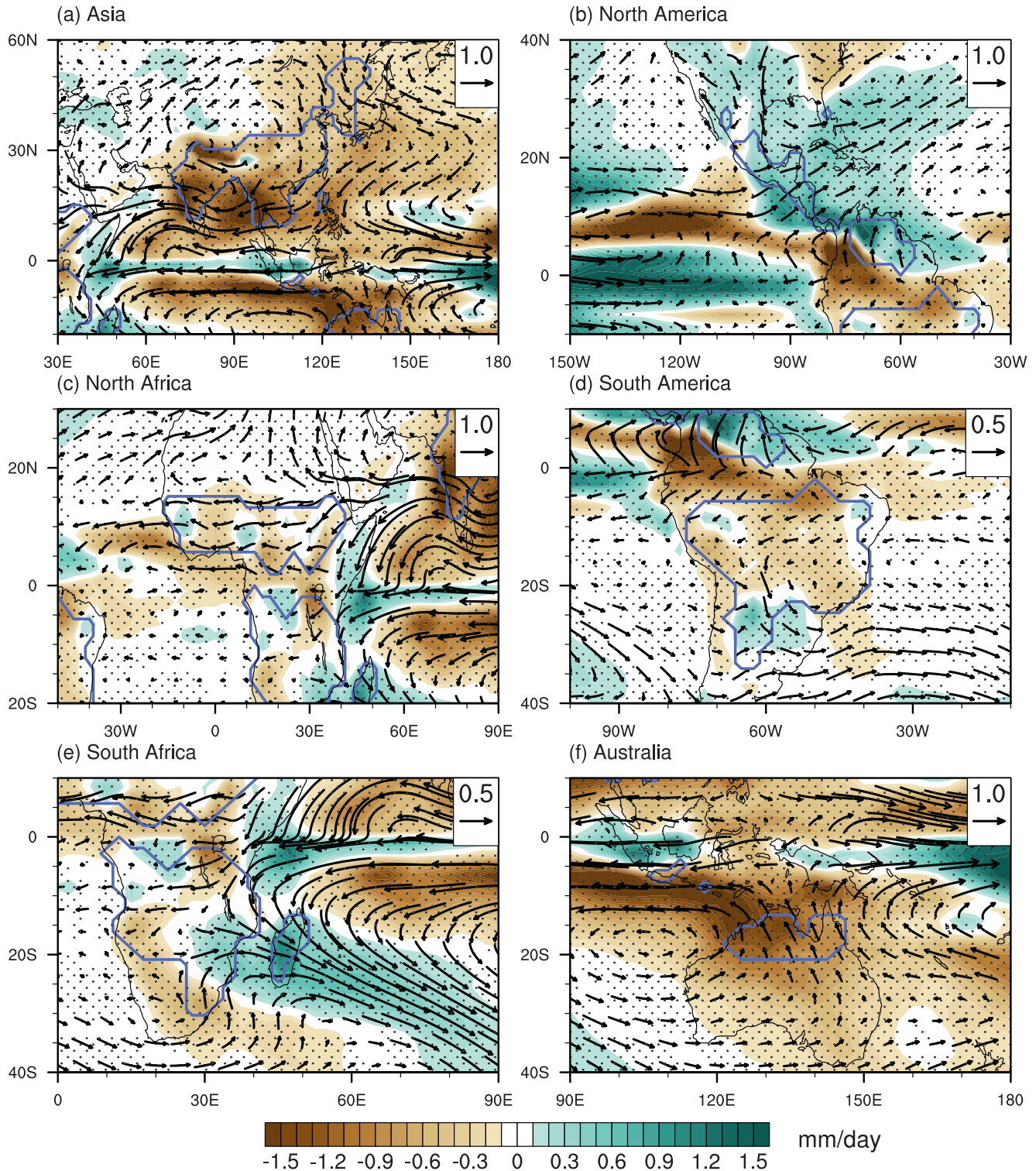
Figure 4. Composite analysis of 850-hPa wind (vectors; \text{m s}^{-1} ) and precipitation (shading; \text{mm day}^{-1} ) anomalies in the local summer of year 0 and year 1 (MJJAS of year 1 for the NH monsoon region; November and December (year 0) and January–March (year 1) for the SH monsoon region) following the large volcanic eruptions. The anomalies are calculated with respect to a 5-year preeruption mean. Dots denote areas that are significant at the 5% level derived from 1,000 Monte Carlo simulations.
