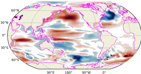
Picontrol Sea surface heighth 31-50 years minus 1-20 years
