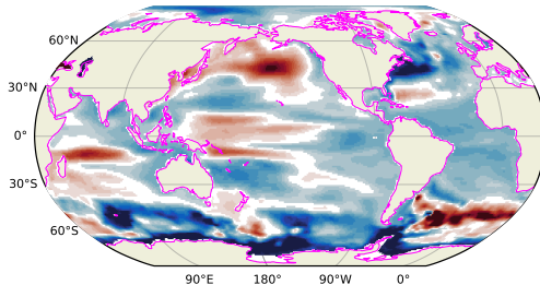
Picontrol with wind nudging Sea surface heighth 31-50 years minus 1-20 years
