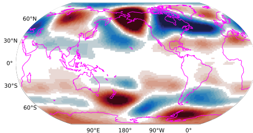
Picontrol with wind nudging 500-hPa geopotential heights 31-50 years minus 1-20 years
