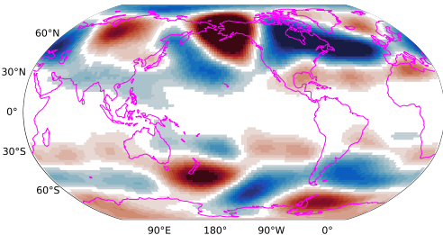
Picontrol 500-hPa geopotential heights 31-50 years minus 1-20 years
