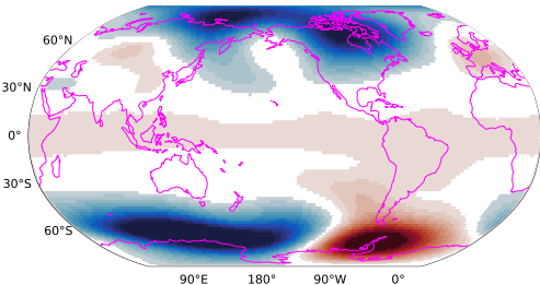
Picontrol 50-hPa geopotential heights 31-50 years minus 1-20 years
