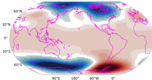
Picontrol with wind nudging 50-hPa geopotential heights 31-50 years minus 1-20 years
