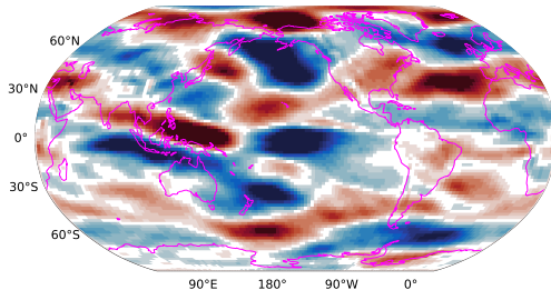
Picontrol with wind nudging 850-hPa zonal winds 31-50 years minus 1-20 years
