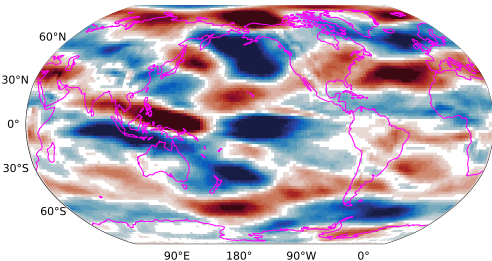
Picontrol 850-hPa zonal winds 31-50 years minus 1-20 years
