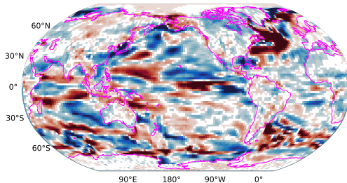
Picontrol with wind nudging total surface heat flux 31-50 years minus 1-20 years
