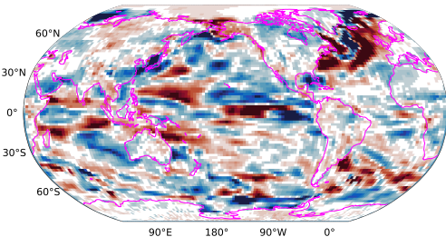
Picontrol total surface heat flux 31-50 years minus 1-20 years
