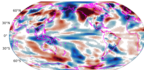
Picontrol with wind nudging Surface meridional stress 31-50 years minus 1-20 years
