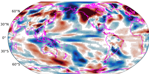
Picontrol Surface meridional stress 31-50 years minus 1-20 years
