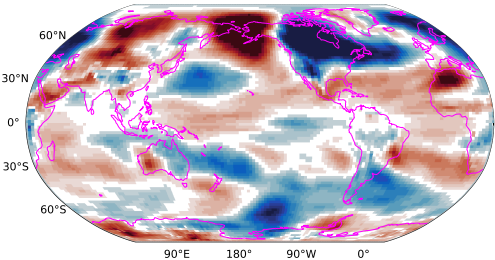
Picontrol 850-hPa atmospheric temperature 31-50 years minus 1-20 years
