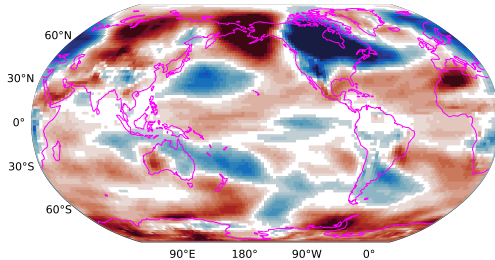
Picontrol with wind nudging 850-hPa atmospheric temperature 31-50 years minus 1-20 years
