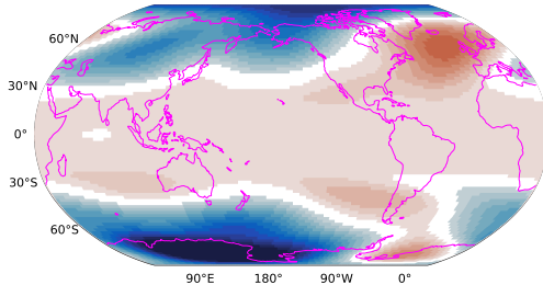
P1control with wind nudging atmospheric temperature @10hPa 31-50 years minus 1-20 years
