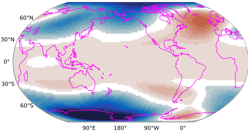
P1control atmospheric temperature @10hPa 31-50 years minus 1-20 years
