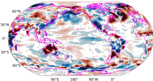
Picontrol surface sensible heat flux 31-50 years minus 1-20 years
