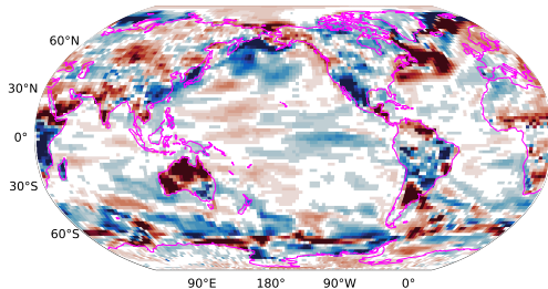
Picontrol with wind nudging surface sensible heat flux 31-50 years minus 1-20 years
