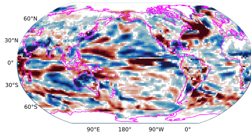
Picontrol with wind nudging surface latent heat flux 31-50 years minus 1-20 years
