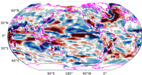
Picontrol surface latent heat flux 31-50 years minus 1-20 years
