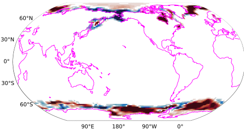
Picontrol sea-ice concentration 31-50 years minus 1-20 years
