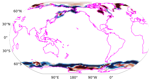
Picontrol with wind nudging sea-ice concentration 31-50 years minus 1-20 years
