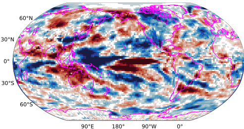
Picontrol net solar flux at top of model 31-50 years minus 1-20 years
