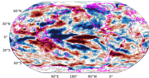
Picontrol with wind nudging net solar flux at top of model 31-50 years minus 1-20 years
