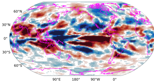
Picontrol with wind nudging net longwave flux at top of model 31-50 years minus 1-20 years
