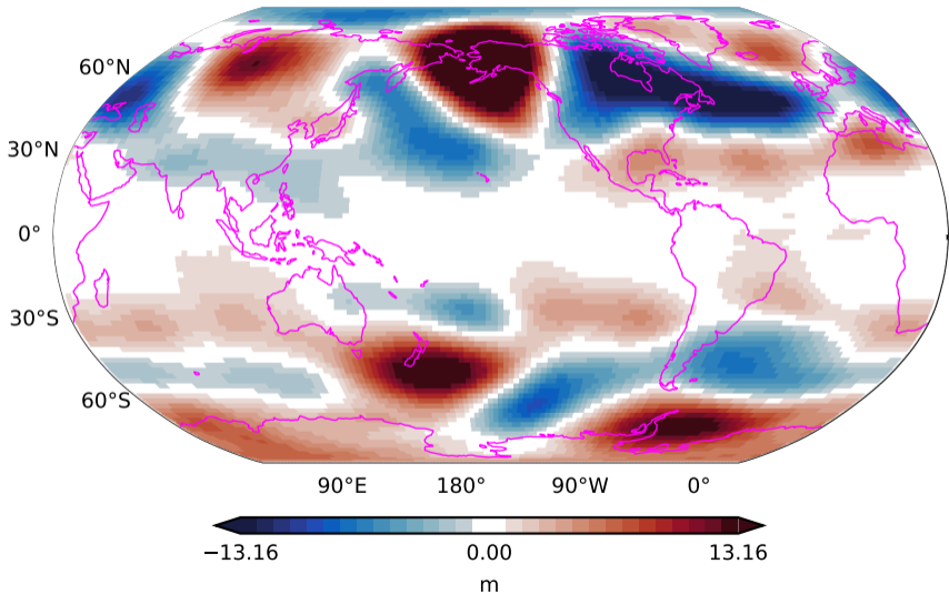
Plcontrol with wind nudging 500-hPa geopotential heights 31-50 years minus 1-20 years
