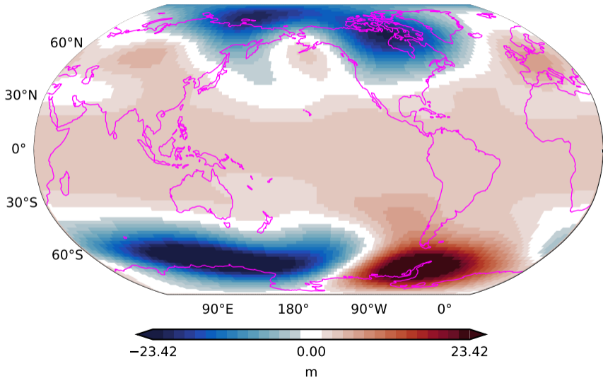
Plcontrol with wind nudging 50-hPa geopotential heights 31-50 years minus 1-20 years
