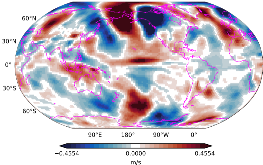
Plcontrol with wind nudging 850-hPa meridional winds 31-50 years minus 1-20 years
