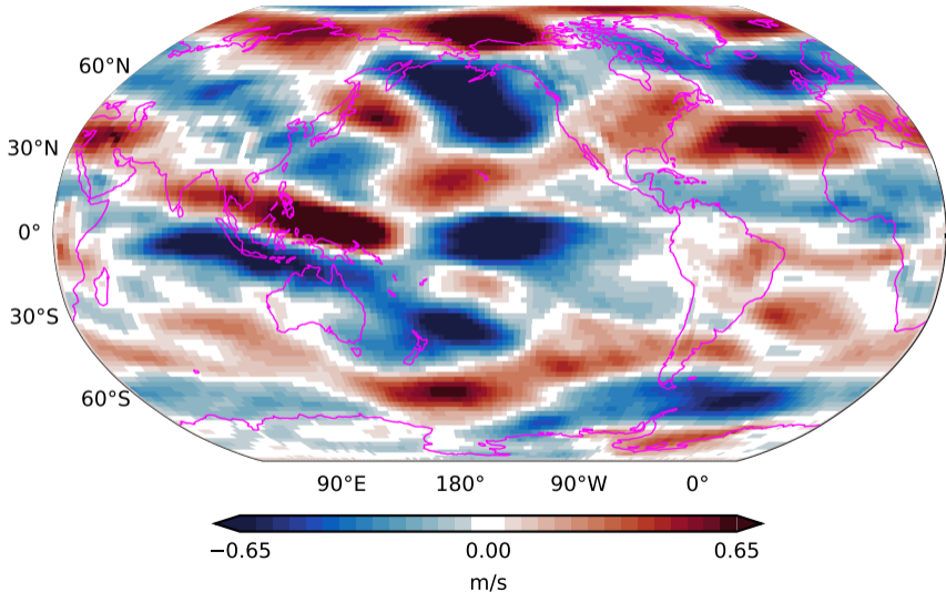
Plcontrol with wind nudging 850-hPa zonal winds 31-50 years minus 1-20 years
