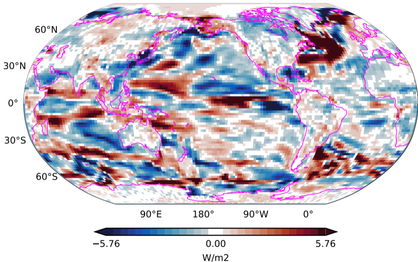
PIcontrol with wind nudging total surface heat flux 31-50 years minus 1-20 years
