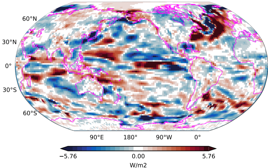
Picontrol total surface heat flux 31-50 years minus 1-20 years
