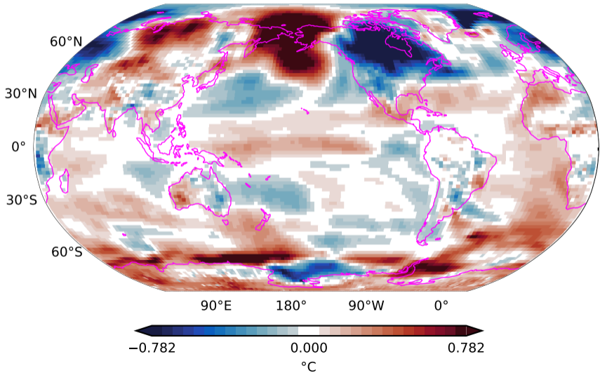
PIcontrol with wind nudging near-surface air temperature 31-50 years minus 1-20 years
