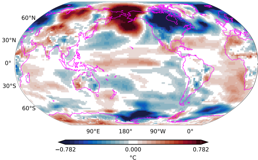
Picontrol near-surface air temperature 31-50 years minus 1-20 years
