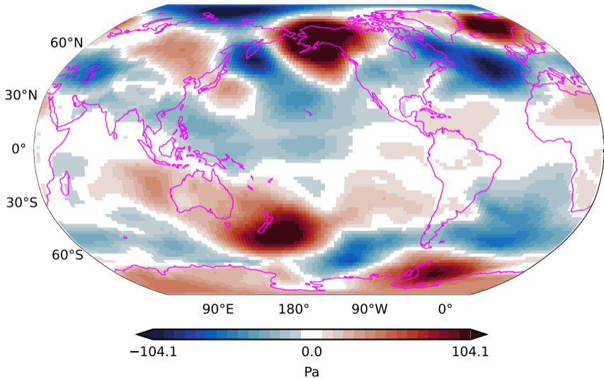
PIcontrol with wind nudging surface pressure 31-50 years minus 1-20 years
