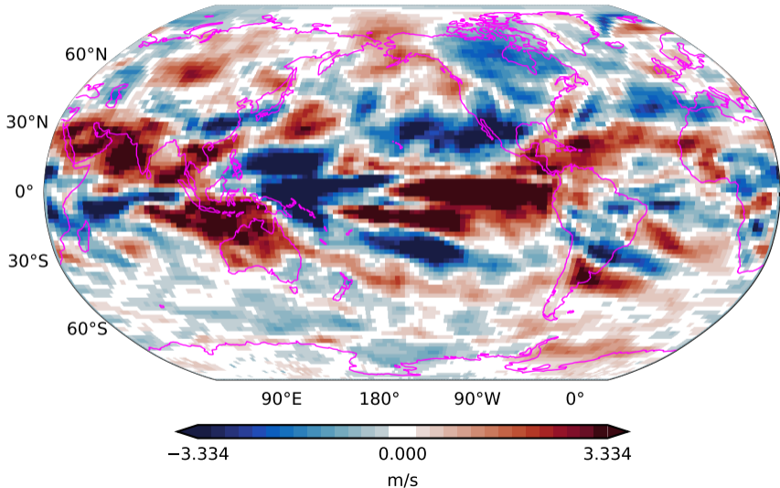
Plcontrol with wind nudging 850-hPa vertical velocity 31-50 years minus 1-20 years
