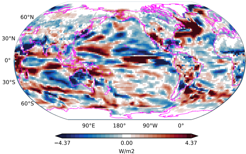
PIcontrol with wind nudging surface latent heat flux 31-50 years minus 1-20 years
