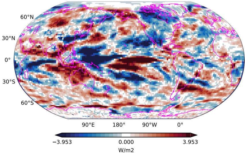
Plcontrol with wind nudging net solar flux at top of model 31-50 years minus 1-20 years
