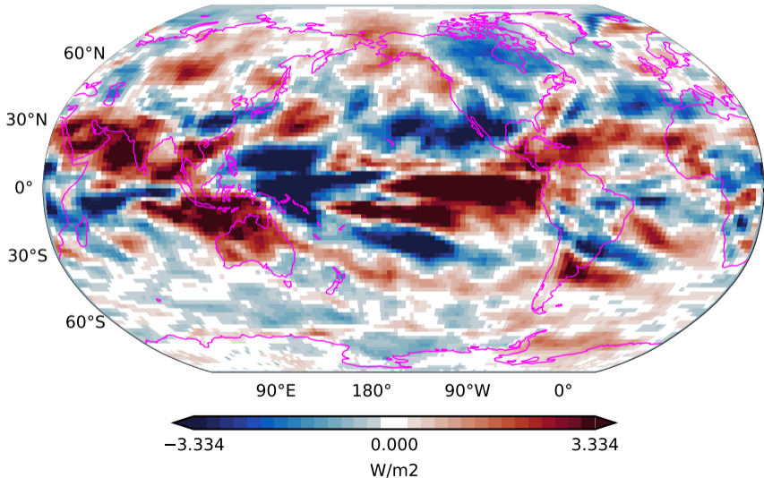
Plcontrol with wind nudging net longwave flux at top of model 31-50 years minus 1-20 years
