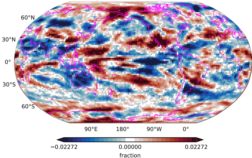
Plcontrol with wind nudging total cloud cover 31-50 years minus 1-20 years
